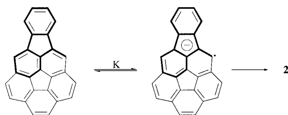
Scheme 2. The dibenzofulvene-like behavior of the radical anion of 1 .
